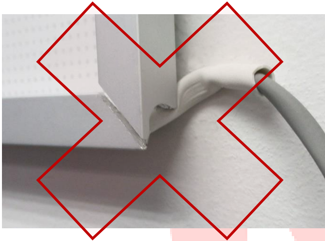
WRONG APPLICATION OF CABLE POSITIONING (Make sure the cable is not under the Dakota Panel)
